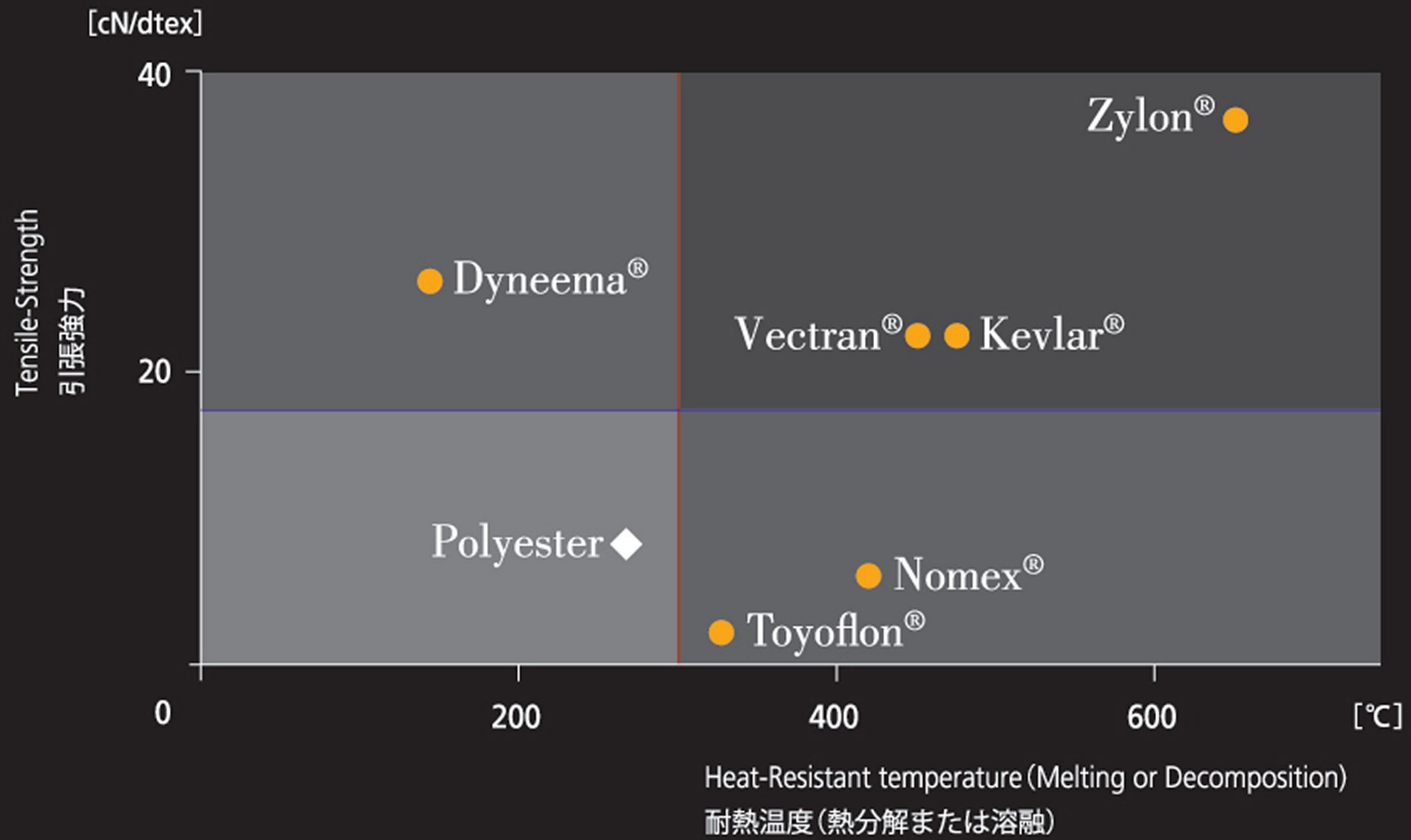
Fig. Relationship between Heat-Resistant and Tensile-Strength 図. 耐熱温度と引張強力の関係
